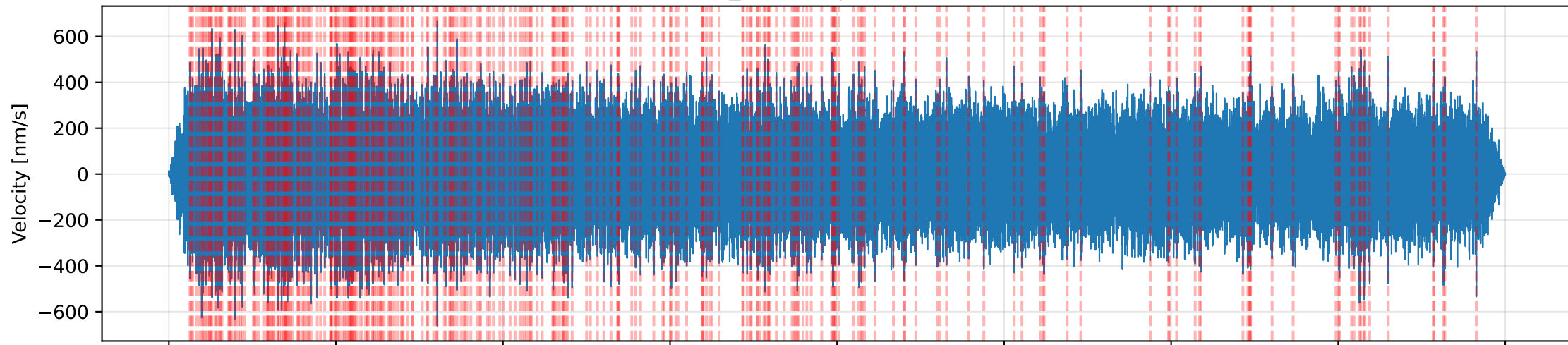
Z_DETECT | 0.1-0.3Hz
