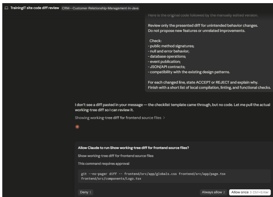
Figure A.3: Diff review request and command-approval step.
