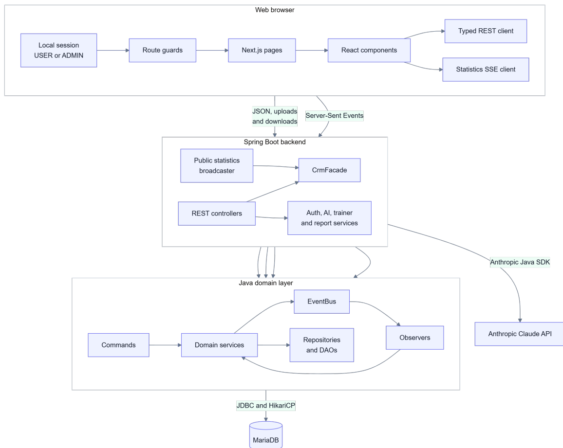
Figure 5.1: Application architecture: the Next.js client, the Spring Boot back end, the pattern-based Java domain layer, the MariaDB database, and the Claude API.
