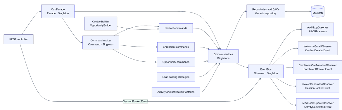
Figure 5.2: Domain patterns and event reactions: the Facade dispatches commands and services, which publish events that fan out to independent observers.
