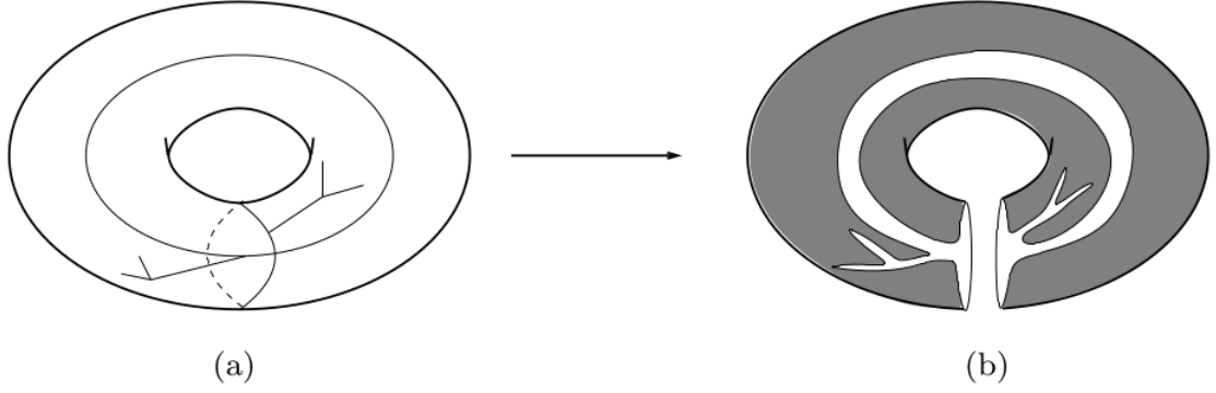
Figure 6.3: Example of a cut in a graph with genus greater than zero. (Borradaile et al. [2014]).
