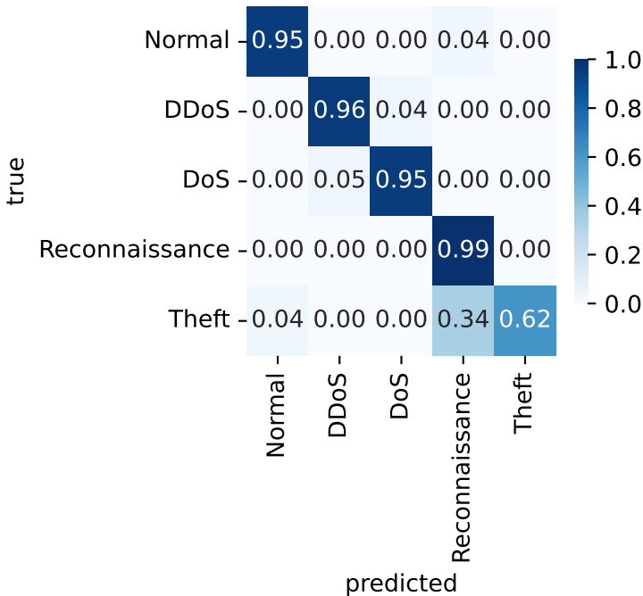
SHIELD student, botiot_category
