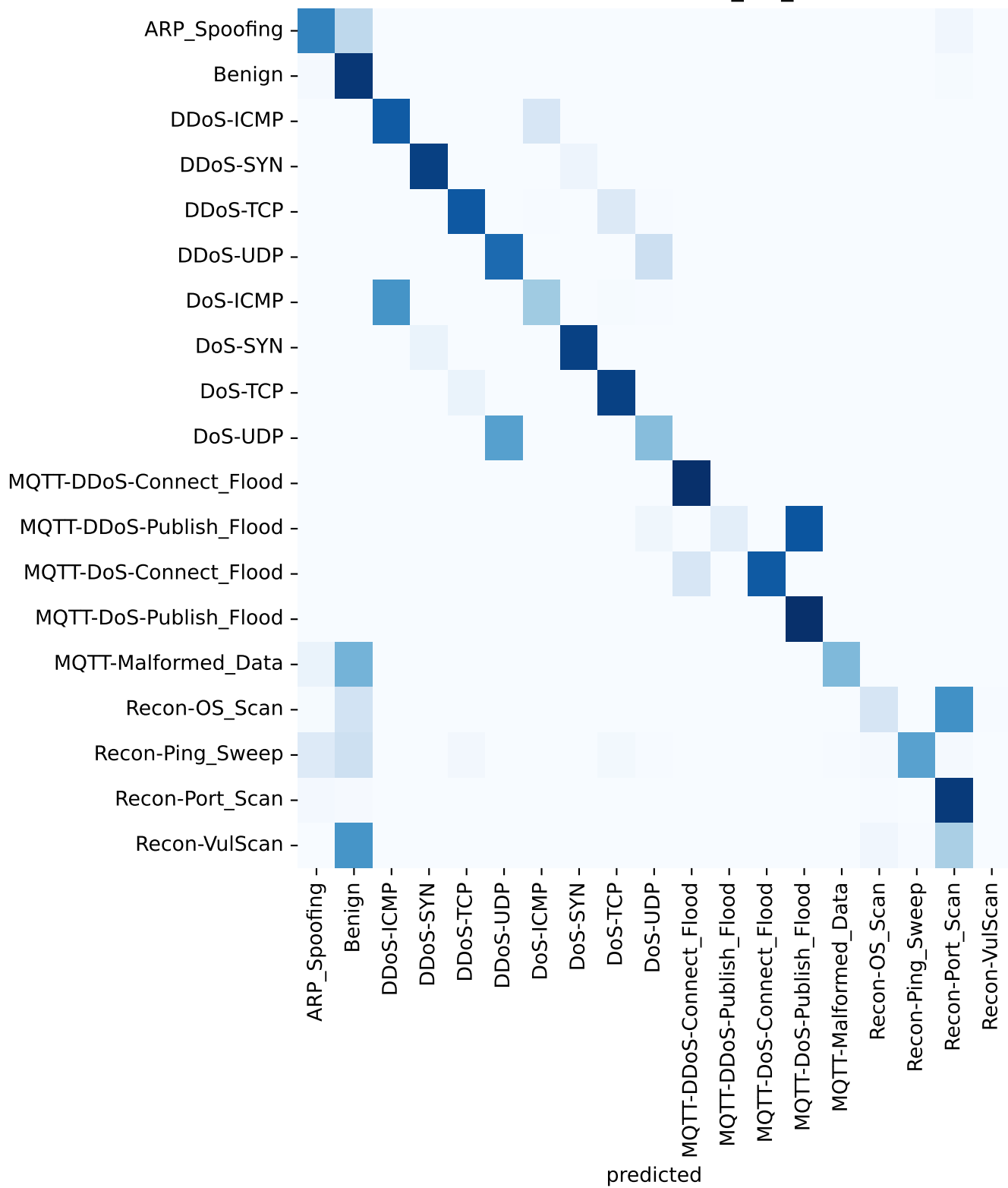
SHIELD student, ciciomt_std_attack
