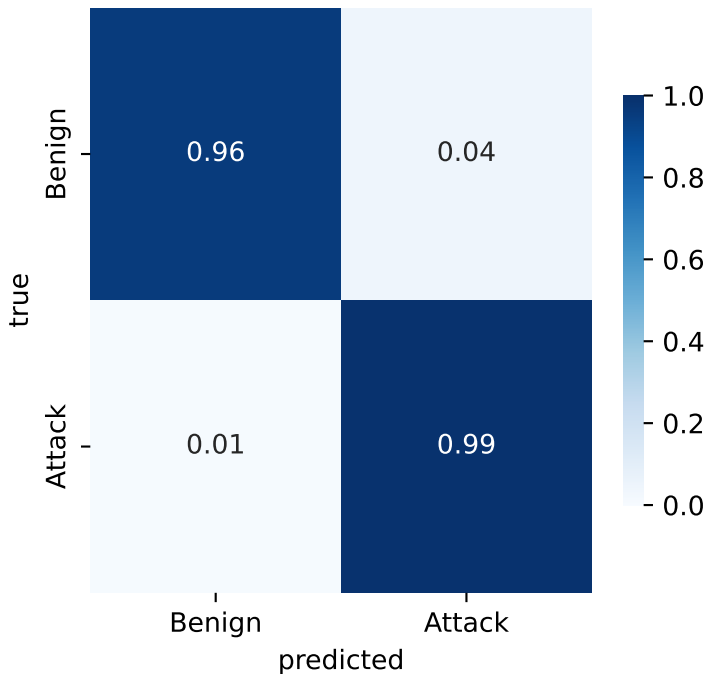
SHIELD student, ciciot_binary
