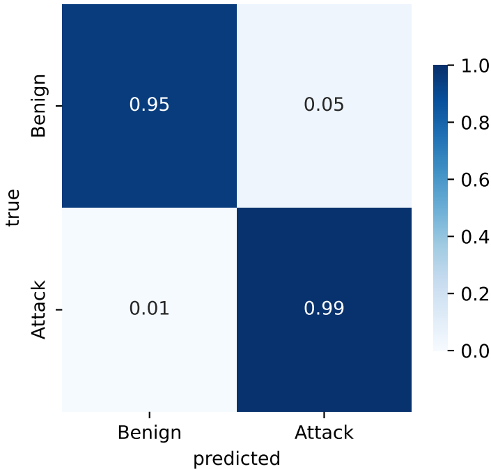
SHIELD student, xciciot_binary
