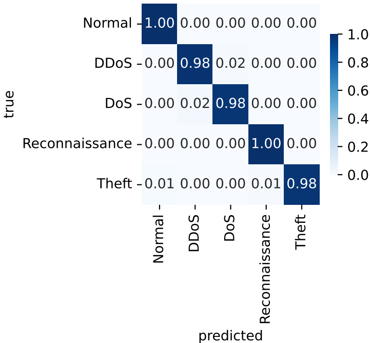
Teacher, botiot_std_category
