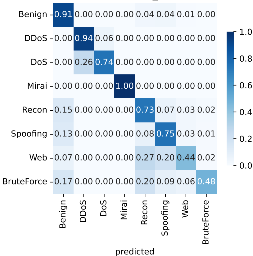
Teacher, ciciot_family
