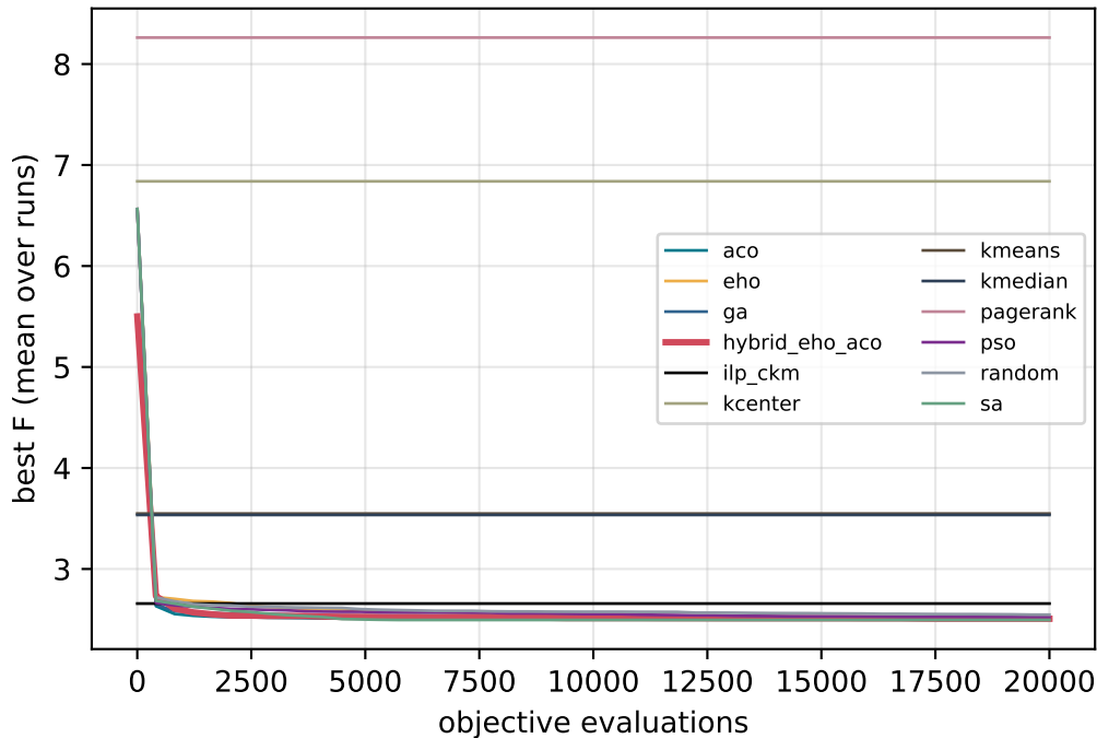
Convergence: syn100, k=4, rho=0.5
