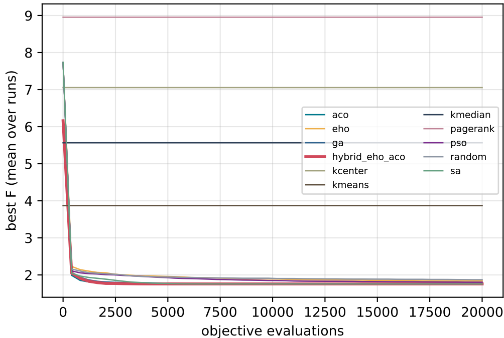
Convergence: syn500, k=4, rho=0.5
