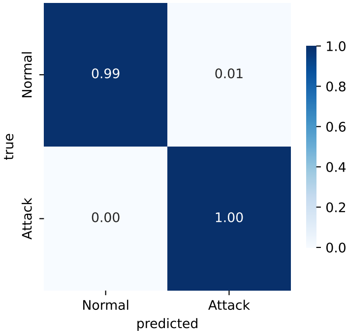
SHIELD student, botiot_binary
