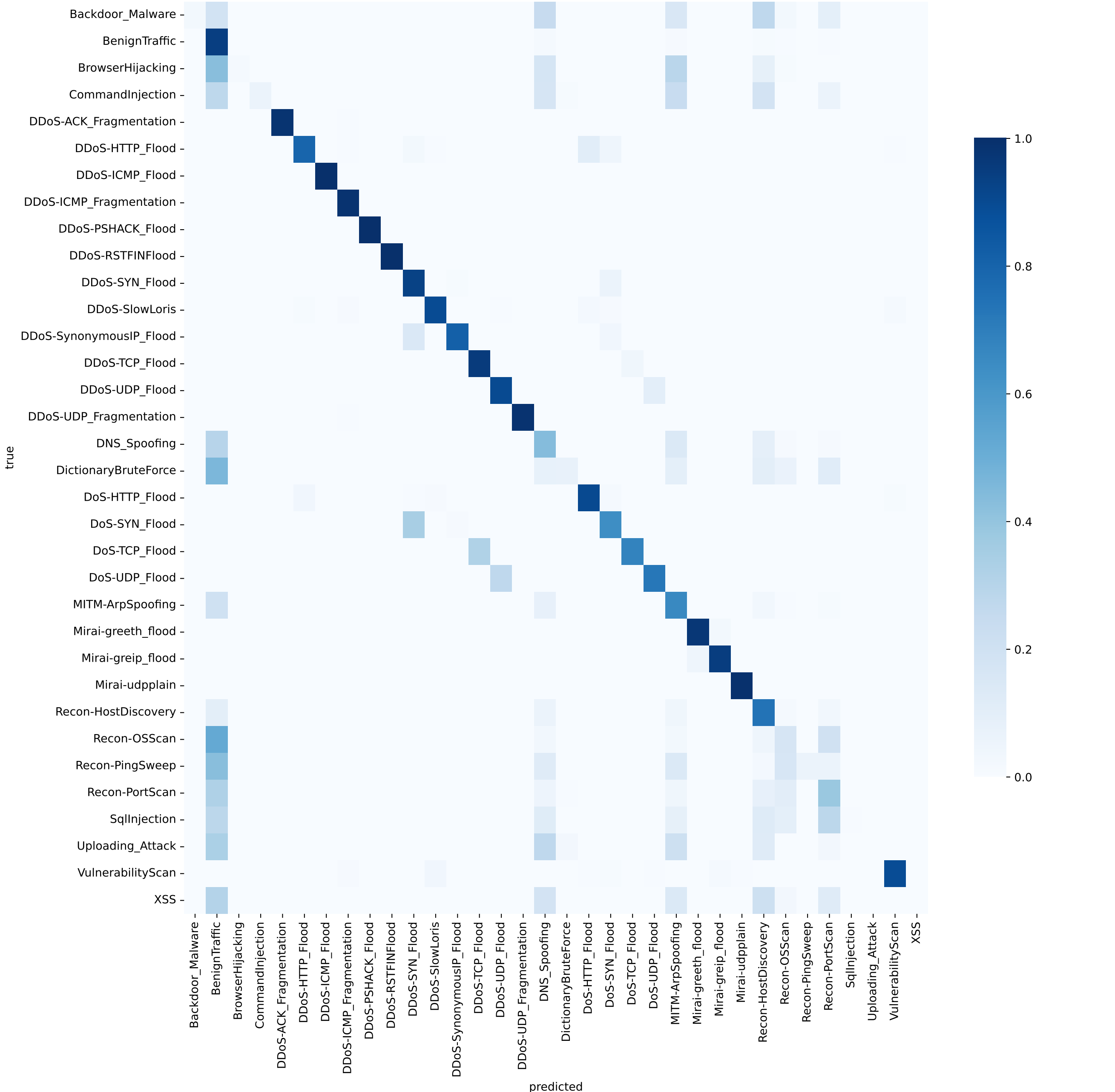
SHIELD student, ciciot_std_class34
