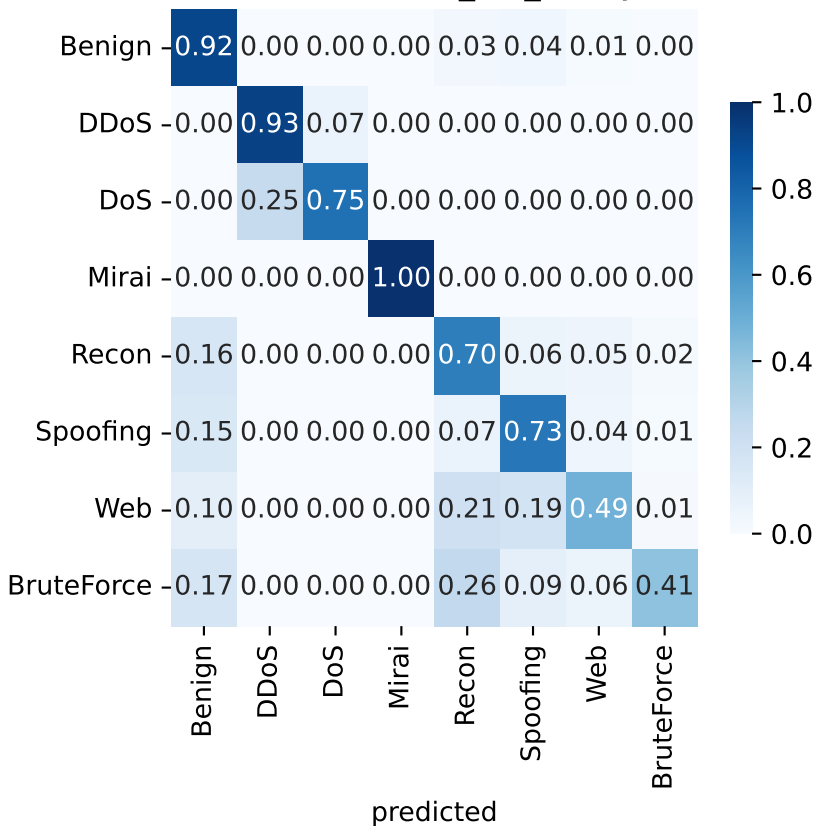
Teacher, ciciot_std_family
