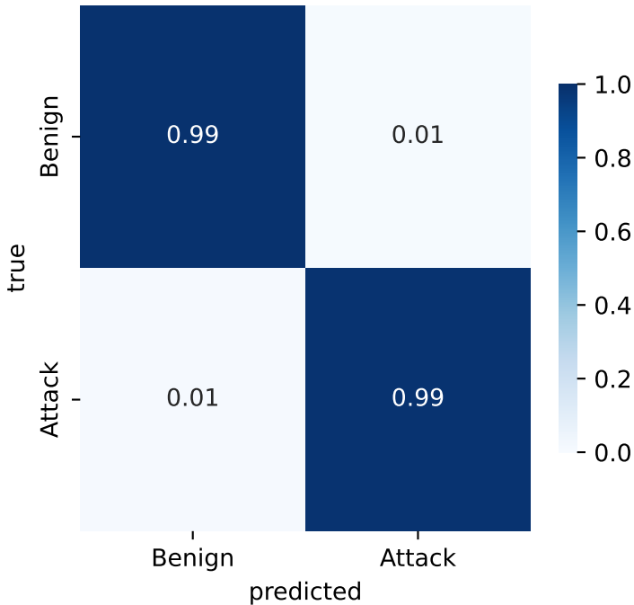
Teacher, xciciot_binary
