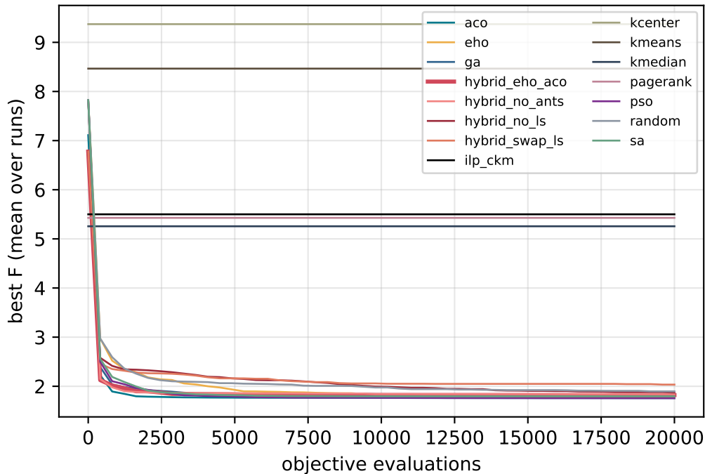
Convergence: Cogentco, k=4 , \rho=0.5
