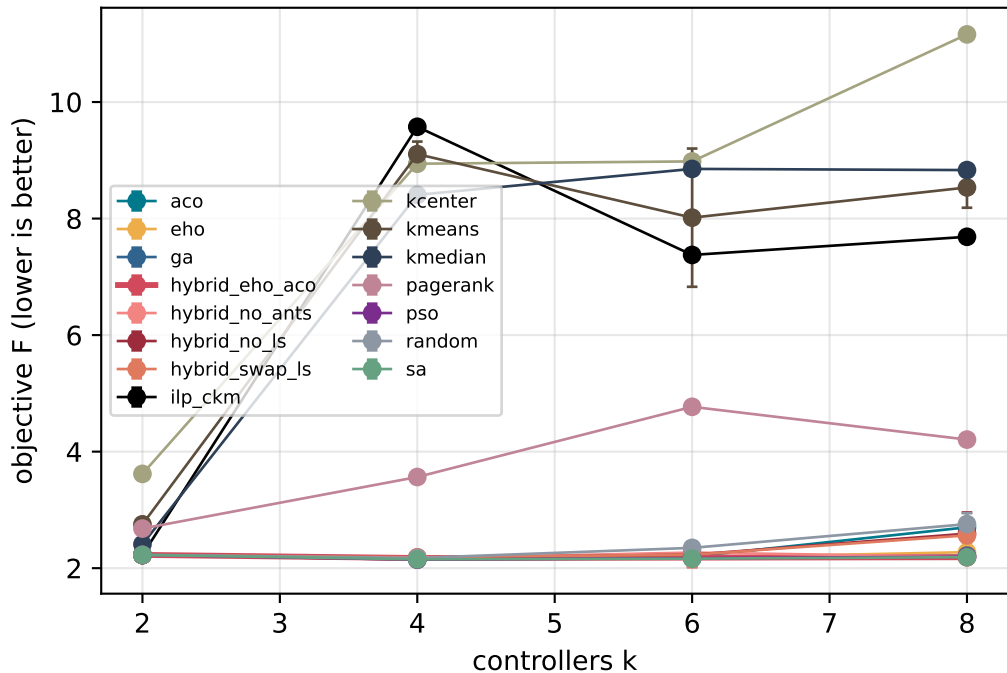
Geant2012, rho=0.5
