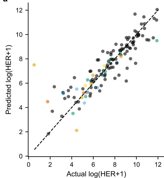
Actual vs predicted (LightGBM) R^2=0.768 , MAE=0.760
