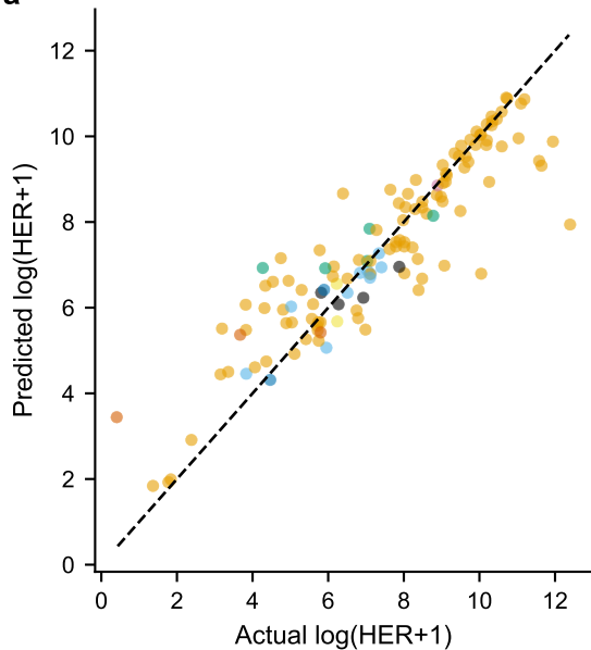
Actual vs predicted (Blending_Ensemble) R^2=0.807 , MAE=0.726
