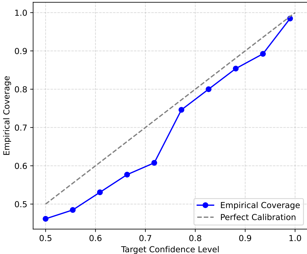
Conformal Prediction Calibration Curve
