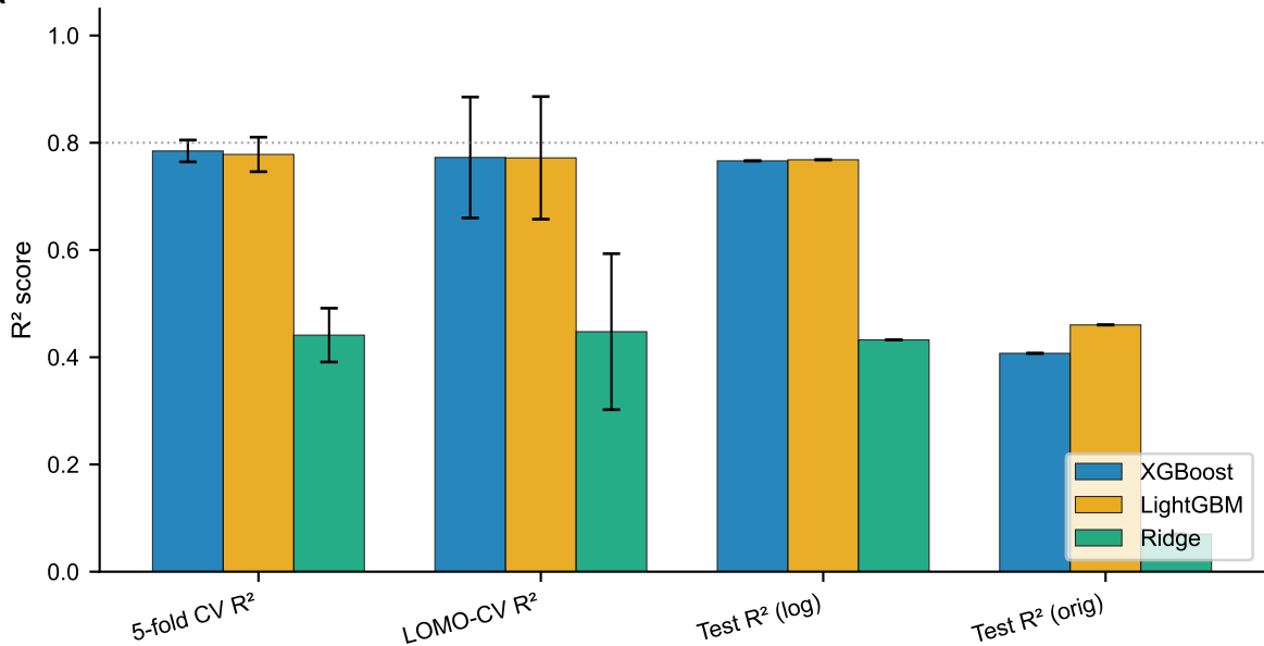
Model performance comparison (best: LightGBM)
