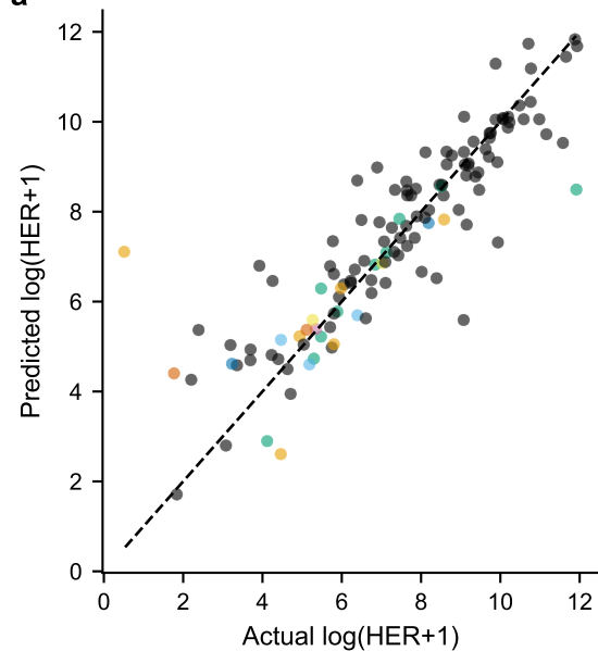
Actual vs predicted (LightGBM) R^2=0.763 , MAE=0.757
