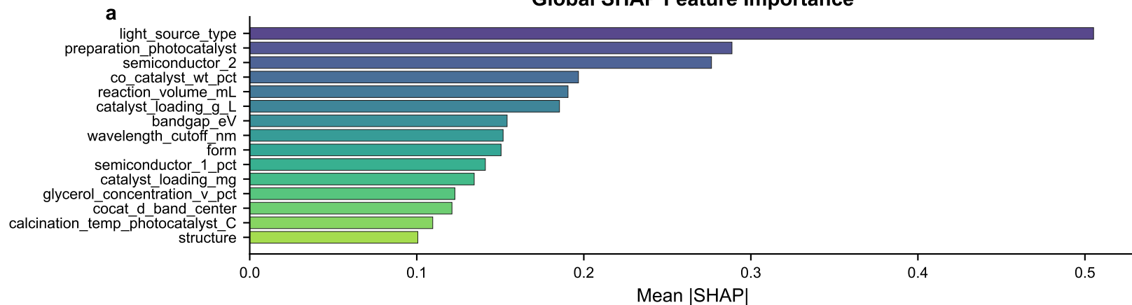
Global SHAP Feature Importance
