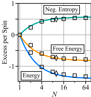
XY Model
