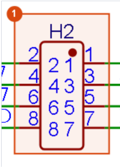
Figure 12 - Sensor module connector H2 (one connector as example)
