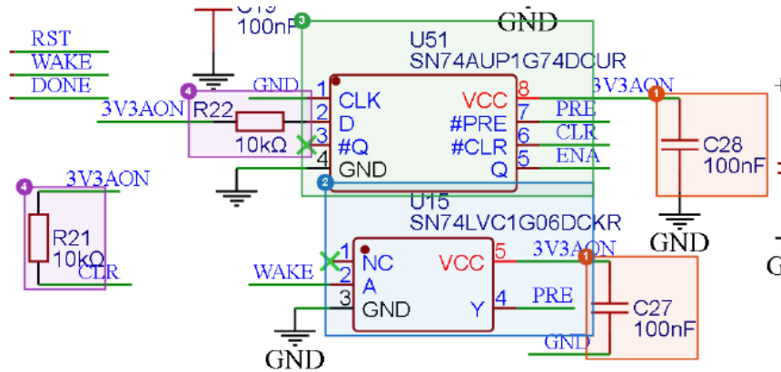
Figure 10 - ENAlatch (U51) and open-drain inverter (U15)
