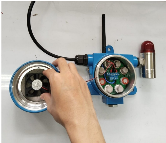
Figure 4-115. GLD V2 - Cover with sampling fan.
