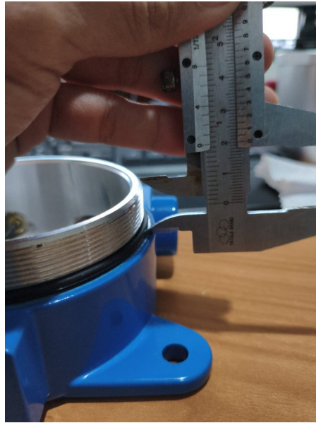
Figure 4-136. GLD V2 - Base neck height from the body shoulder — caliper ≈20.2 mm.
