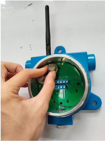
Figure 4-107. GLD V2 - Sensor modules fitted. Sensor modules installed on the terminal board positions.
