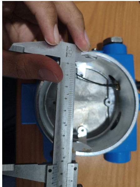
Figure 4-131. GLD V2 - Base inner bore — caliper ≈84.7 mm.
