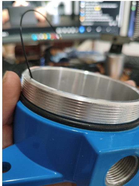
Figure 4-127. GLD V2 – Cover thread and side-entry thread.
