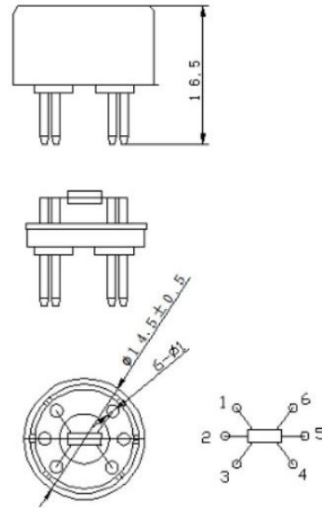
Fig1. Sensor Structure
