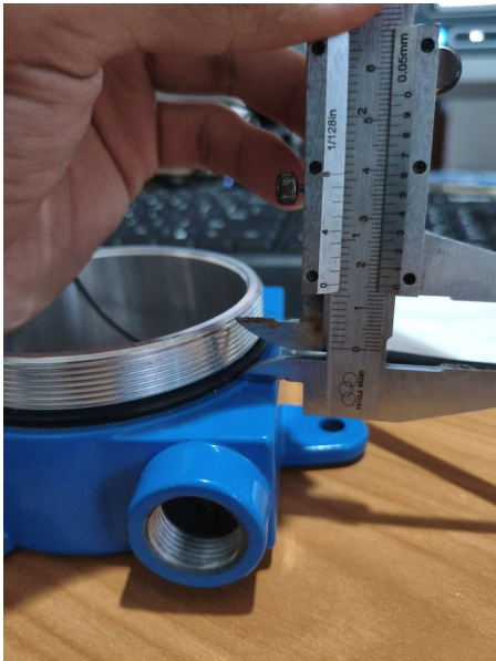
Figure 4-130. GLD V2 - Threaded neck height — caliper ≈14.8 mm.
