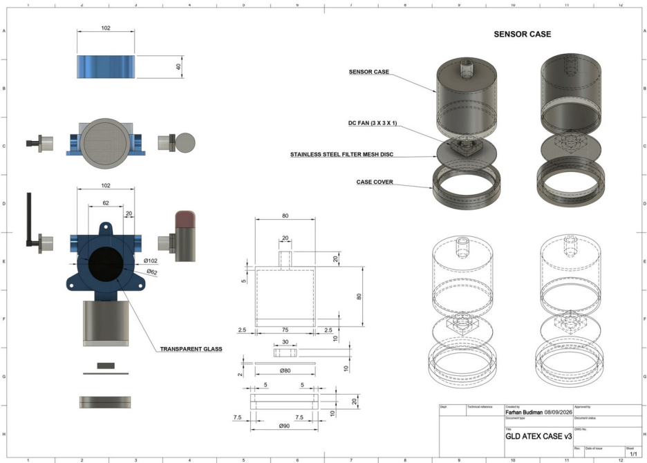
“GLD ATEX CASE v3” — dimensioned enclosure drawing sheet
