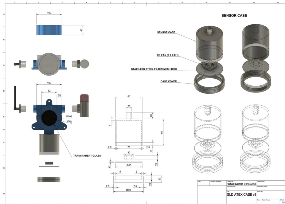
"GLD ATEX CASE v3" dimensioned drawing sheet (8 Sep 2026) — internal contingency/alternate enclosure design, not the confirmed production enclosure.
