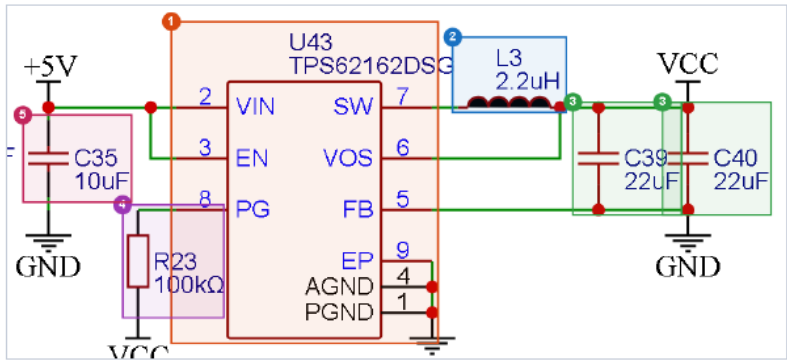
Figure 7 - 5 V to 3.3 V buck (U43)
