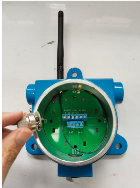
Figure 4-106. GLD V2 - Sensor module being inserted. Sensor module plugged into one of the eight headers.
