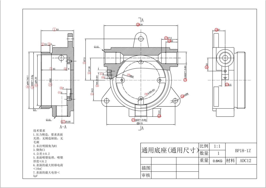
“Universal Base” BP18-1Z — supplier reference drawing
