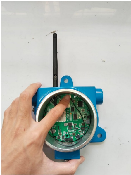
Figure 4-103. GLD V2 - Antenna lead connected to the main board. U.FL coaxial connector of the antenna lead plugged onto the main board.
