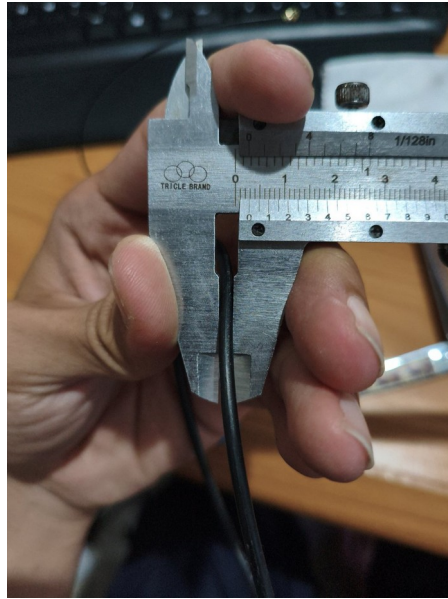
Figure 4-132. GLD V2 – Cover O-ring — cord cross-section 2.70 mm. Black rubber O-ring of the cover-to-base joint measured across its cord: reading 2.70 mm.
