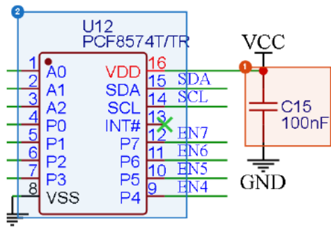
Figure 14 - Sensor module enable I/O expander (U12)
