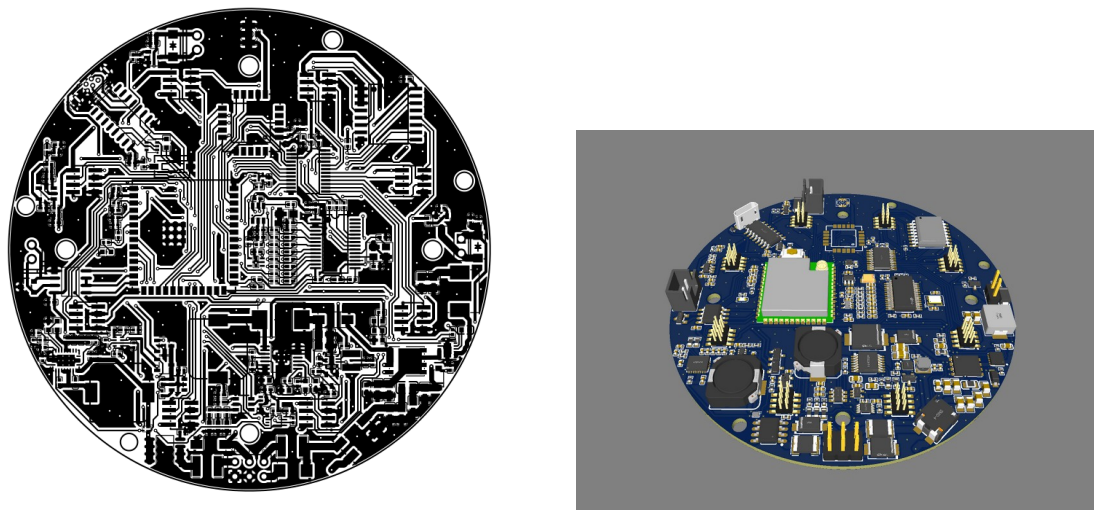
Main board PCB layout (top copper) and 3D populated render
