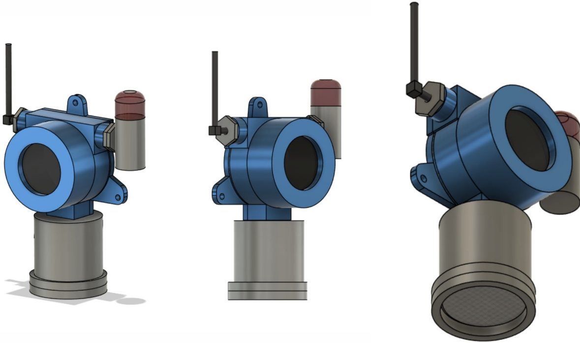
M-B1. GLD ATEX CASE v3 — sheet 1: isometric views of the assembled detector
