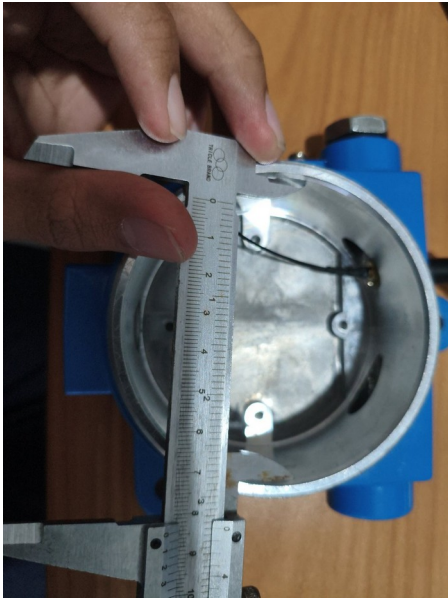
Figure 4-131. GLD V2 – Base inner bore — caliper \approx 84.7 mm. Inside jaws across the bore of the base at the top of the neck: reading \approx 84.7 mm.
