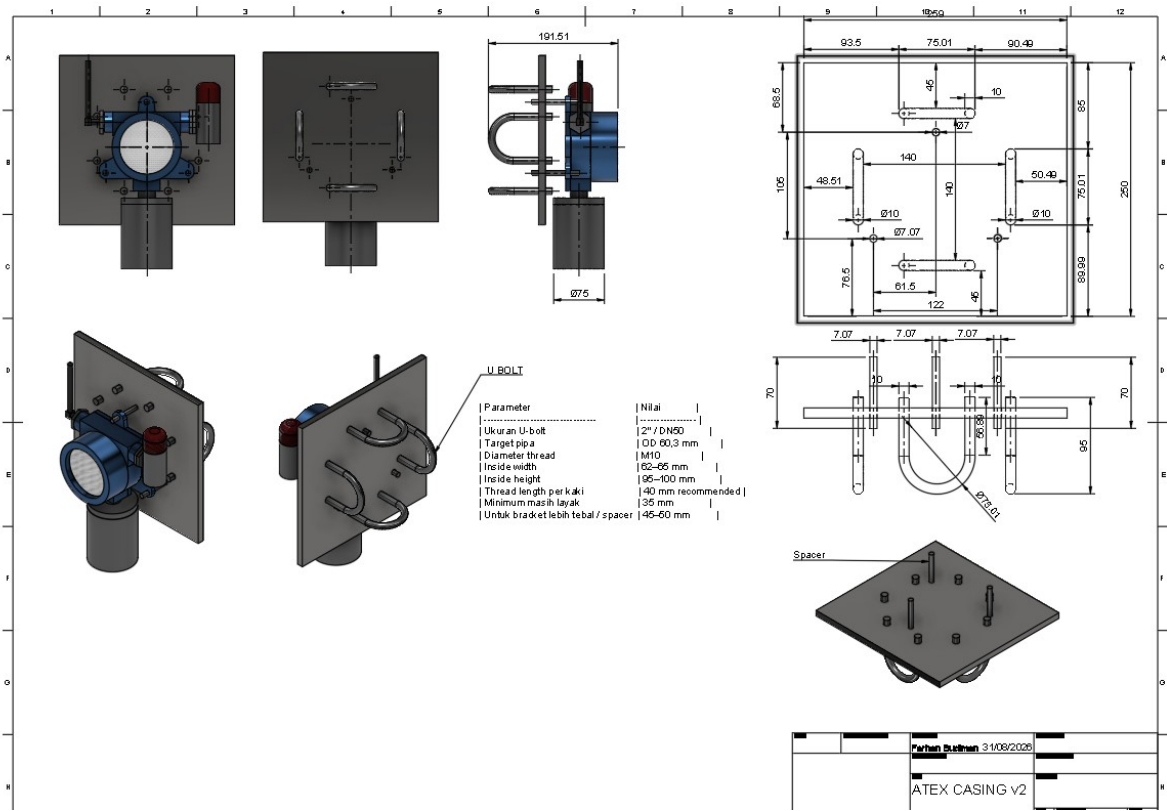
Enclosure envelope & mounting bracket — dimensioned drawing sheet
