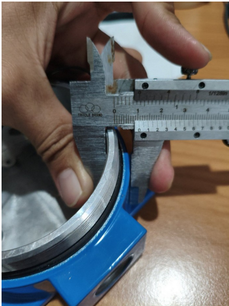
Figure 4-128. GLD V2 - Base neck wall at the O-ring — caliper 10.50 mm. Vernier caliper (0.05 mm) across the neck wall at its root, just above the O-ring: reading 10.50 mm.
