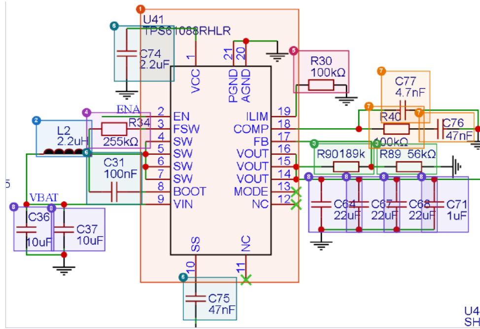
Figure 6 - Battery boost to 5 V (U41, TPS61088)
