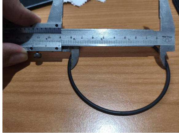
Figure 4-134. GLD V2 - Cover O-ring — outer diameter ≈91.0 mm.
