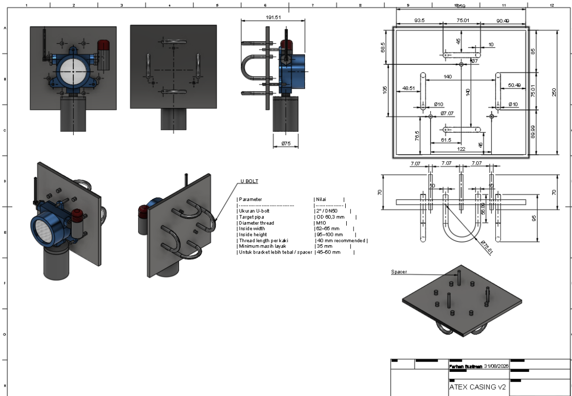
Enclosure envelope & L-bracket/U-bolt mounting assembly — dimensioned drawing sheet (drafted 31 Aug 2026, from a STEP solid model).
