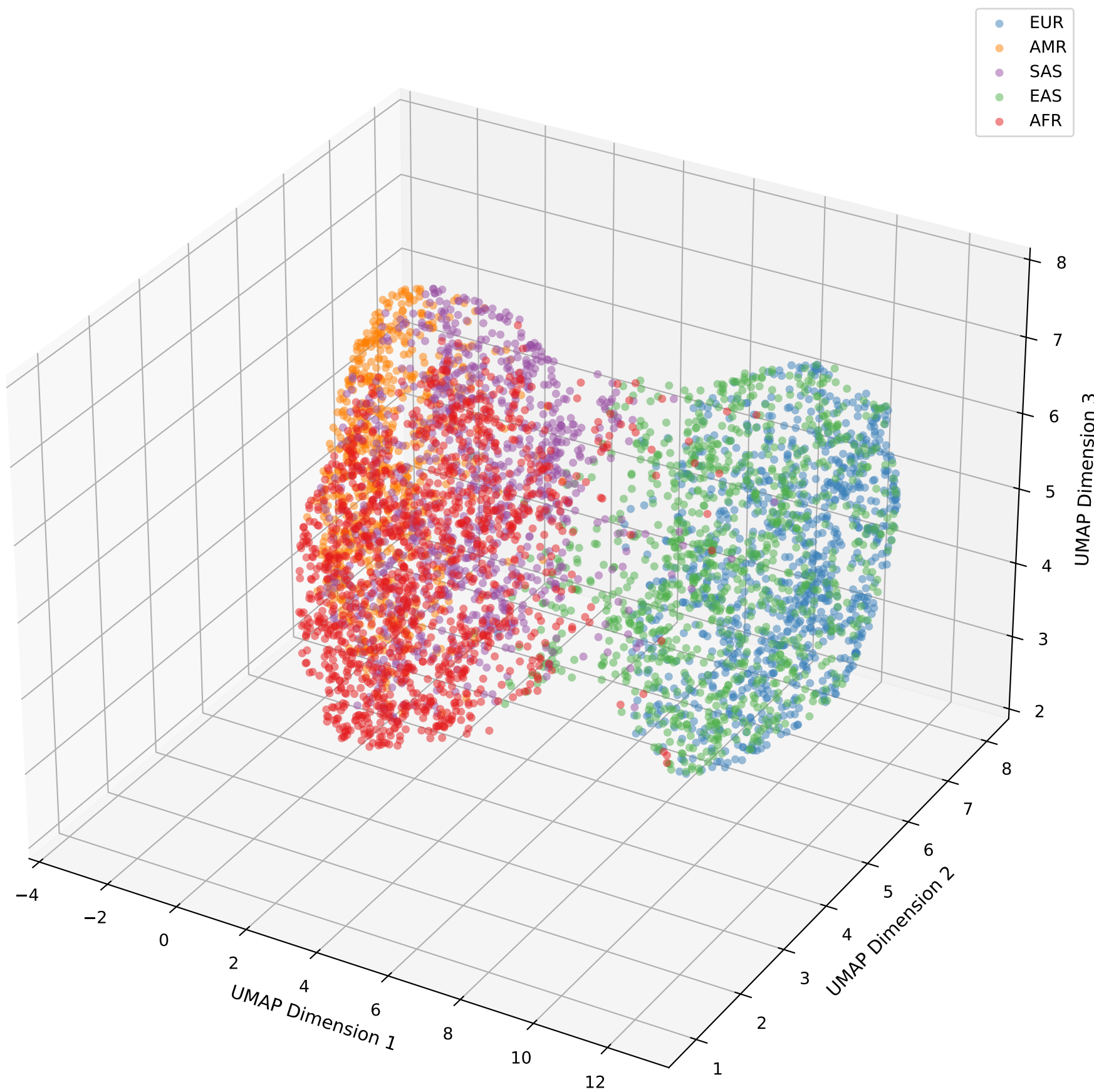
3D UMAP: Ancestry Clusters
