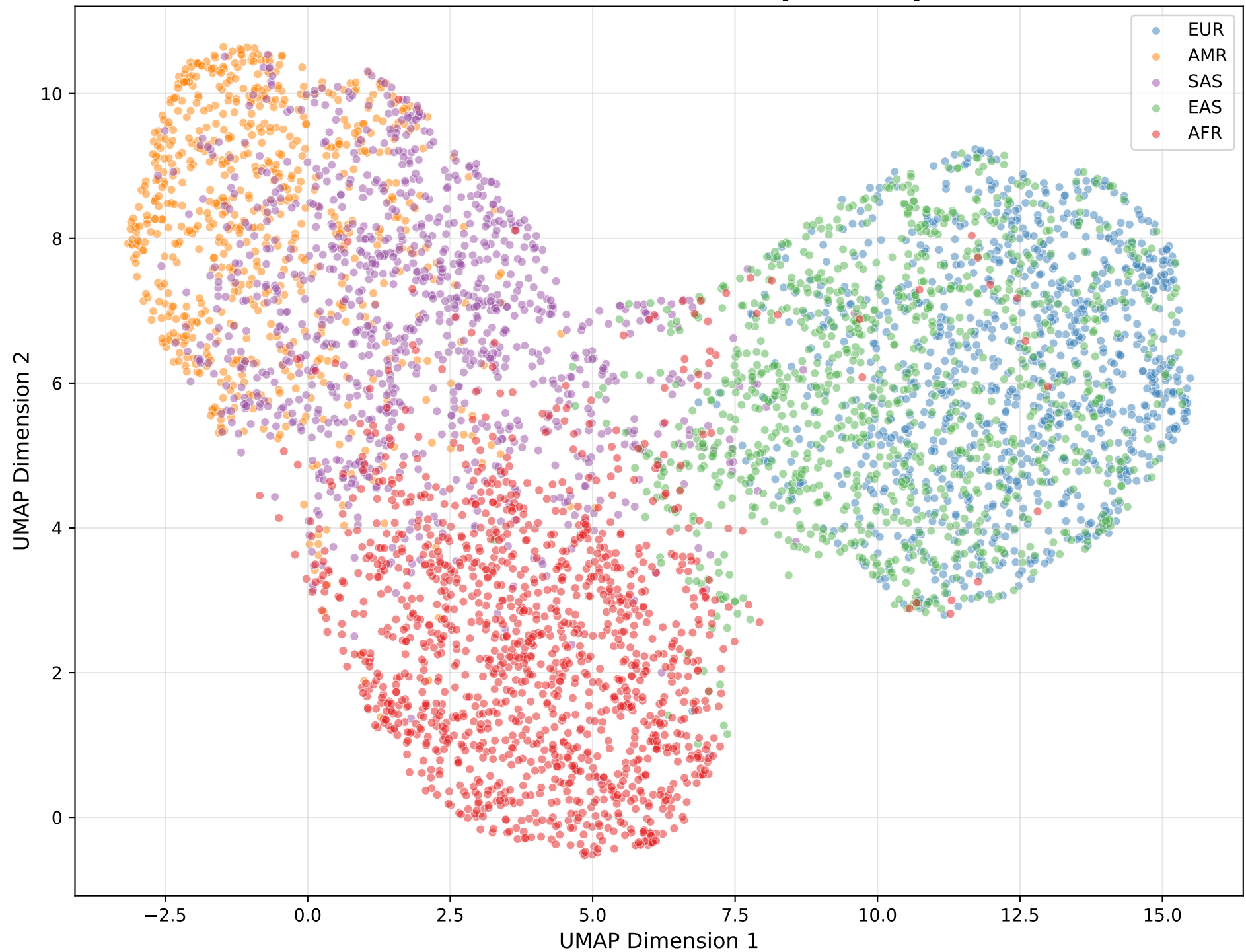
UMAP: Genetic Risk + SES by Ancestry
