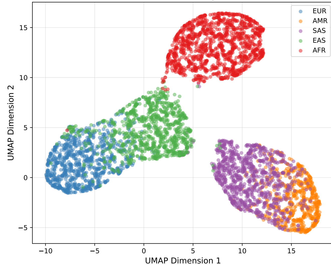
UMAP: Clear Ancestry Clusters
