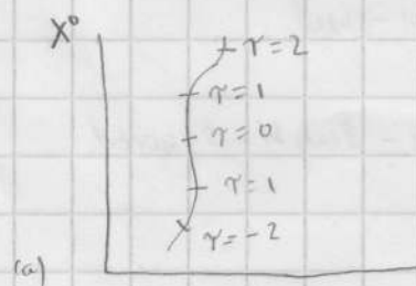
a) point particle \Rightarrow World line
