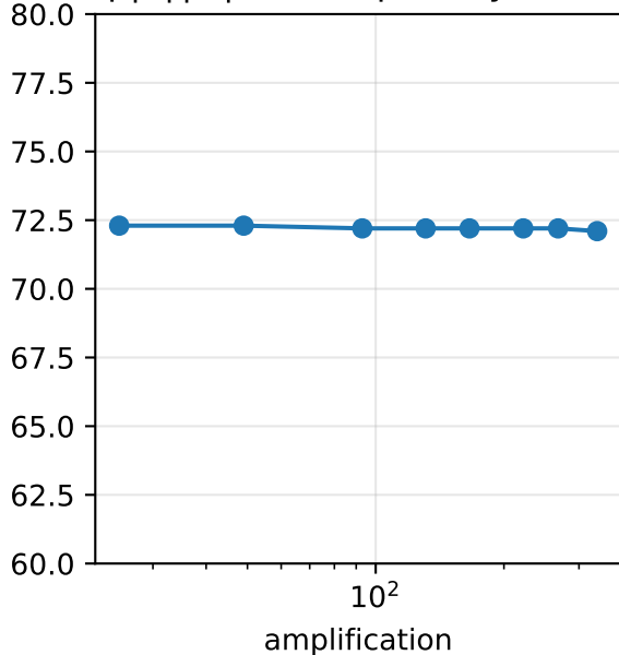
\sup|u| |x'| (KNSS quantity, T-free)
