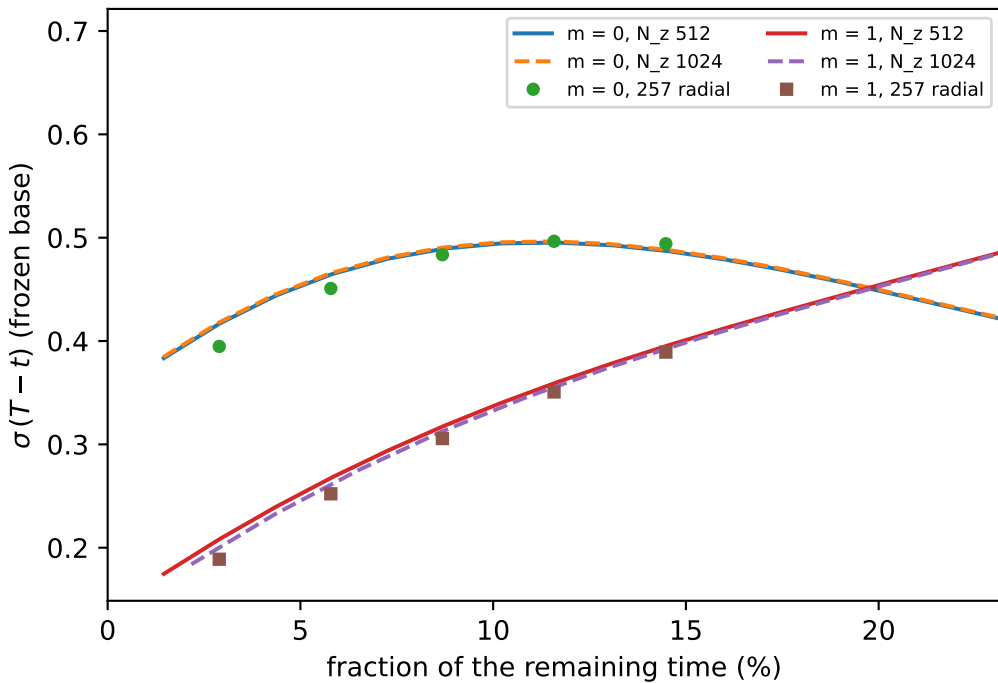
Resolution pairs, Euler x28 ( T_E = 0.002278 )
