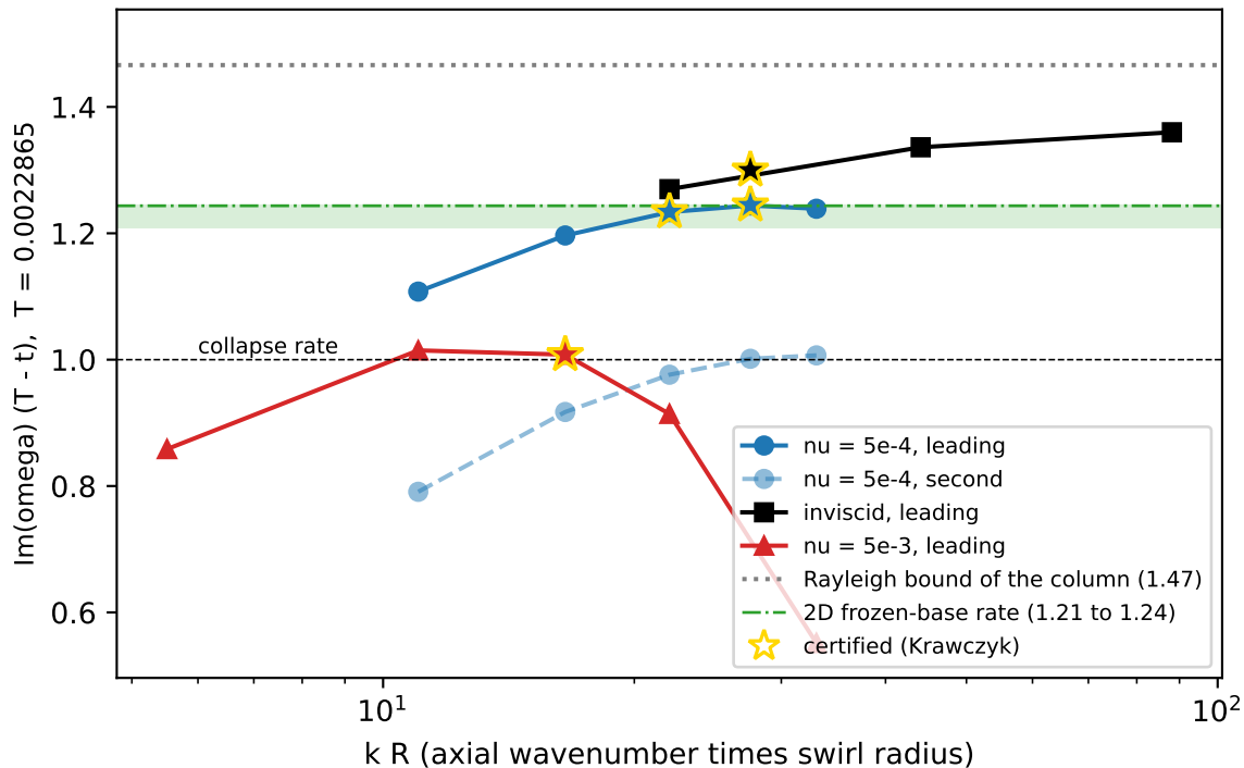
Columnar normal modes of the front column ( m = 1 ), x144 state
