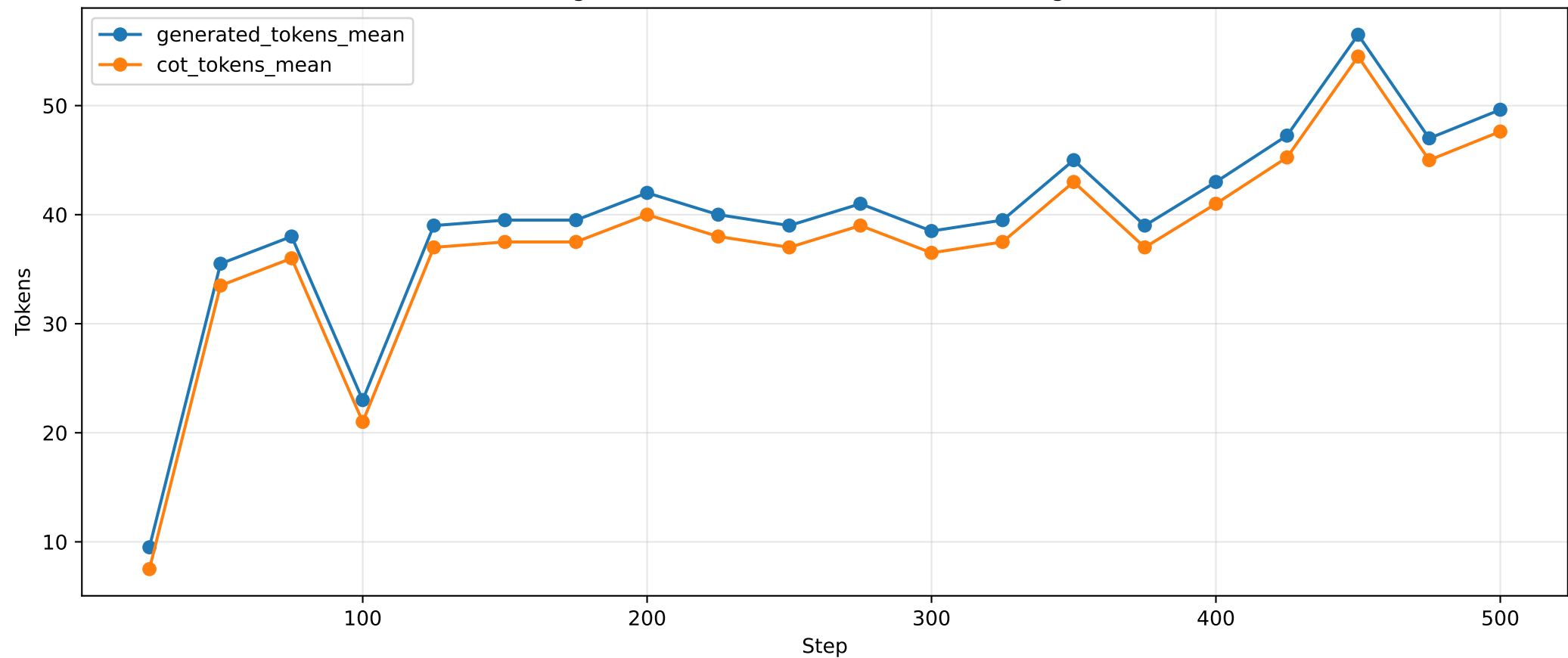
Mean generated tokens and CoT tokens during rollout
