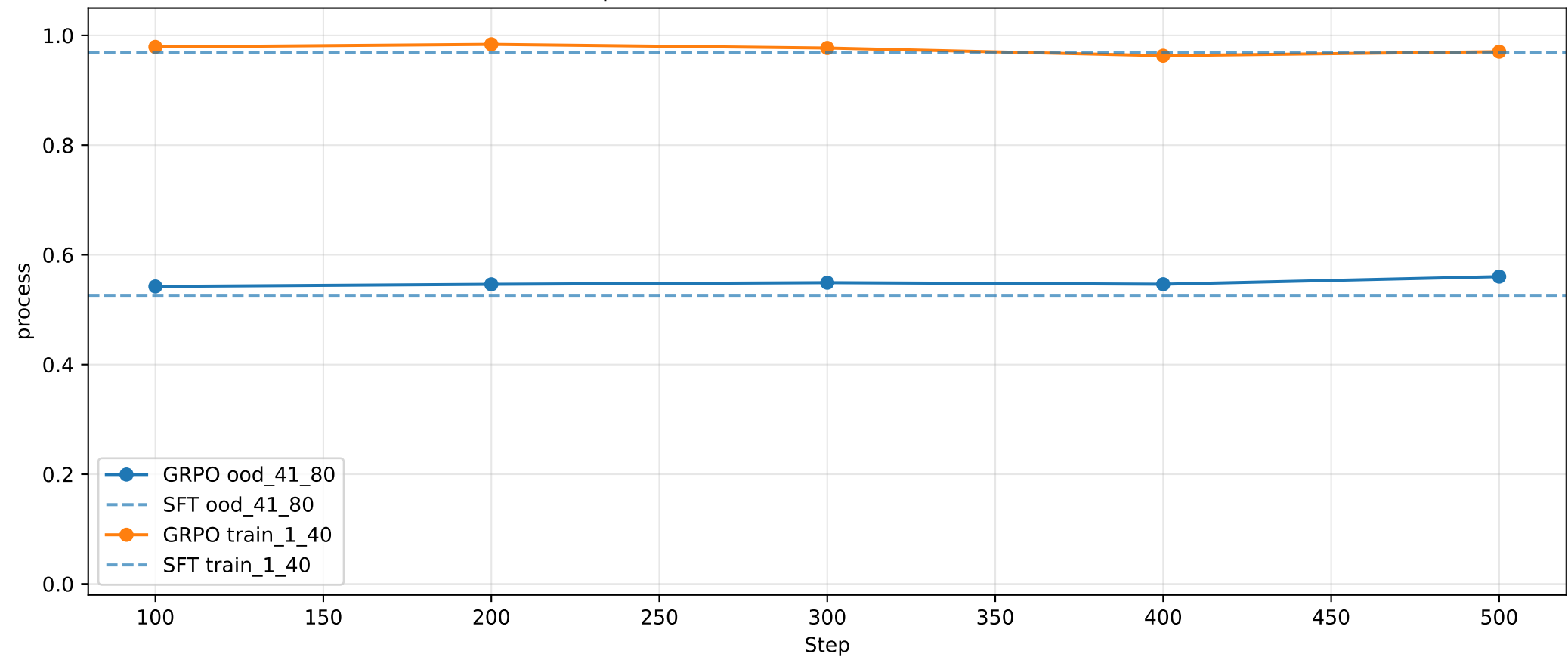
Eval process: GRPO curriculum vs SFT baseline
