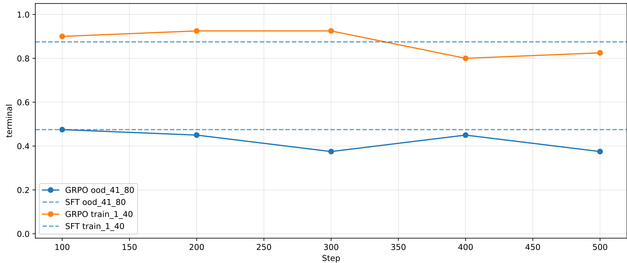
Eval terminal: GRPO curriculum vs SFT baseline
