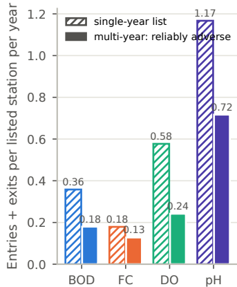
b List turnover, 2018-2024
