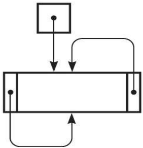
(b) listHead
