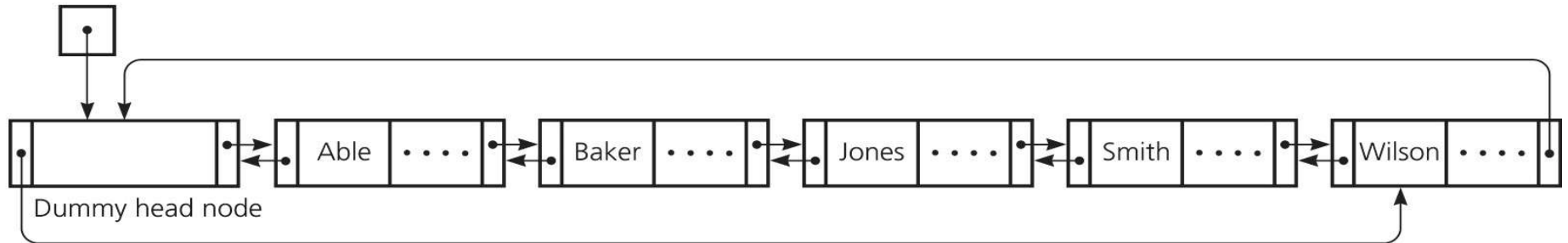
(a) listHead
