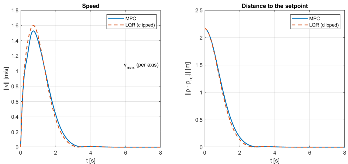
Figure 9: Toy model, Model 2 step 9: receding-horizon MPC versus input-clipped LQR on the learned model.
