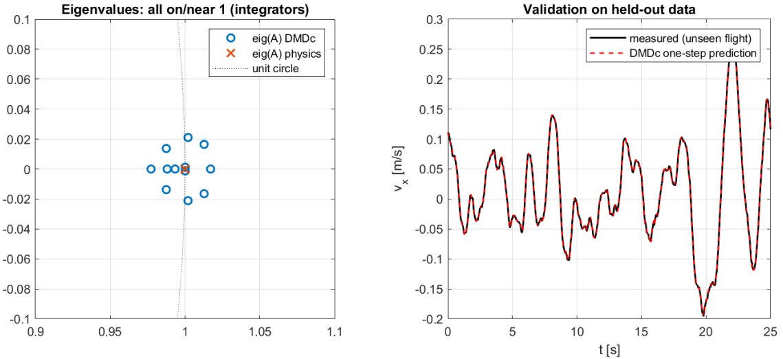
Figure 7: Toy model, Model 2 step 2. Left: eigenvalues of the learned and physical A , all at or near 1 (integrators). Right: one-step predictions on a flight that was not used for learning.
