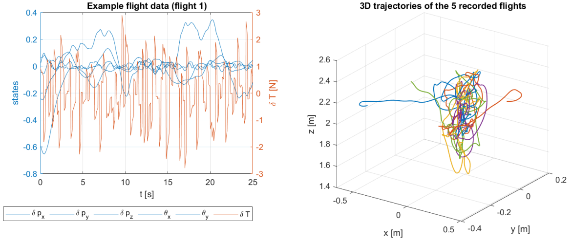
Figure 6: Toy model, Model 2 step 1: example time histories and the 3D tracks of the five recorded flights.
