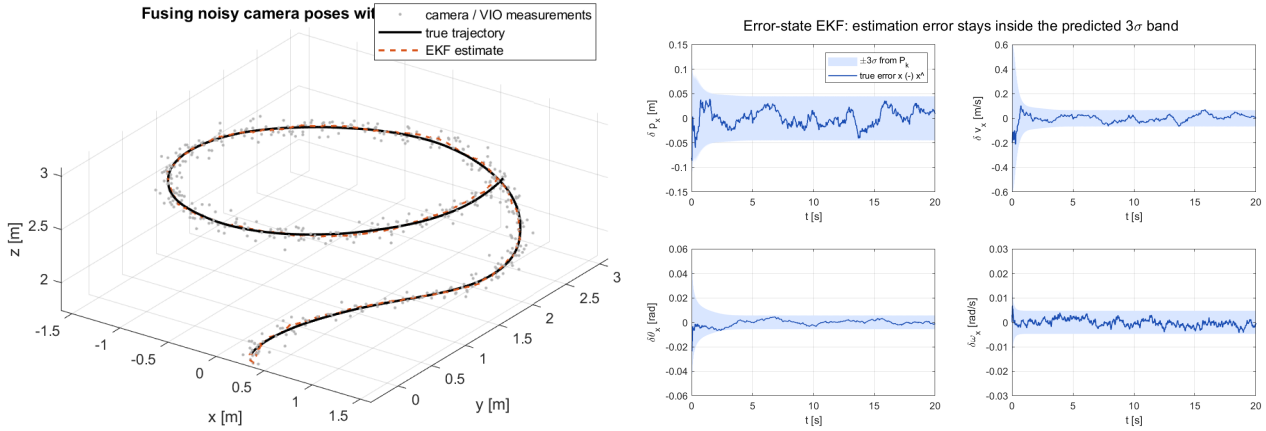
Figure 3: Toy model, Model 1 step 4. Left: noisy camera positions (grey), truth (black) and EKF estimate. Right: estimation errors stay inside the \pm 3\sigma band computed from P_k .
