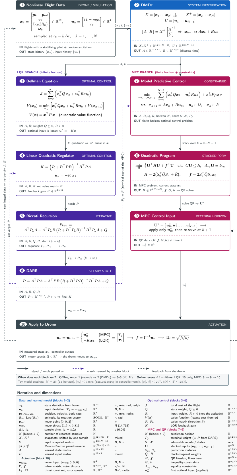
Figure 2: Model 2 equation flow: data-driven linear model (DMDc) followed by two optimal-control branches, LQR (left) and MPC (right), that meet when the command is applied to the drone.
