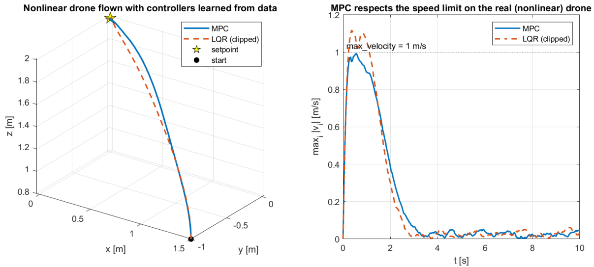
Figure 10: Toy model, Model 2 step 10: the nonlinear drone flown by controllers that were designed on a model learned from data.
