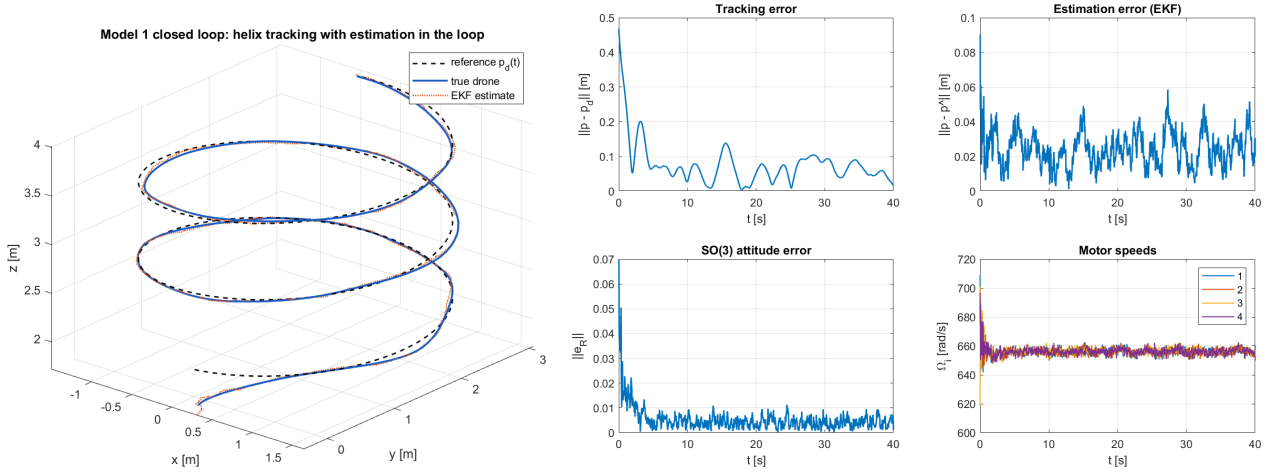
Figure 5: Toy model, Model 1 step 8: the complete loop (truth \rightarrow sensors \rightarrow EKF \rightarrow blocks 5–7 \rightarrow allocation \rightarrow truth) tracking a climbing helix in wind. After the transient: tracking RMSE 6.8 cm, estimation RMSE 2.6 cm, motor speeds 619–709 rad/s.
