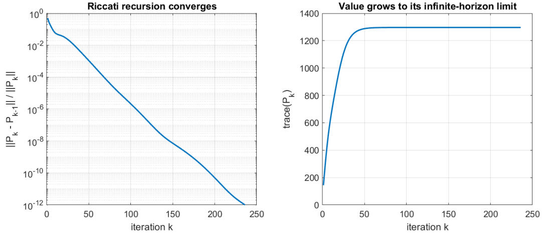
Figure 8: Toy model, Model 2 step 5: convergence of the Riccati recursion for the learned drone model.
