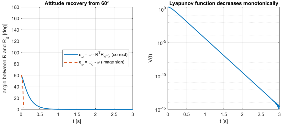
Figure 4: Toy model, Model 1 step 7. Left: recovery from 60° with the corrected and the original sign of e_\omega . Right: the Lyapunov function V decreases monotonically with the corrected law.
