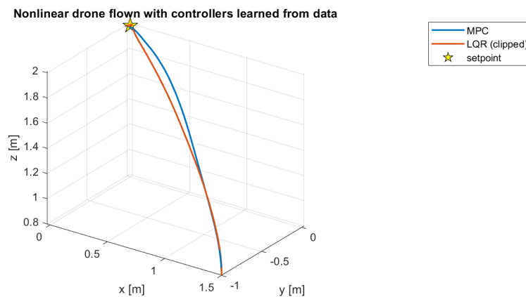
Figure 14: The nonlinear drone flown by MPC and by LQR, both designed only from recorded data.
