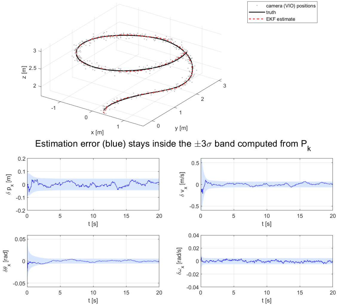
Figure 6: Top: noisy camera positions (grey dots), truth (black) and EKF estimate (red, dashed). Bottom: estimation errors (blue) stay inside the \pm 3\sigma band computed from P_k .
