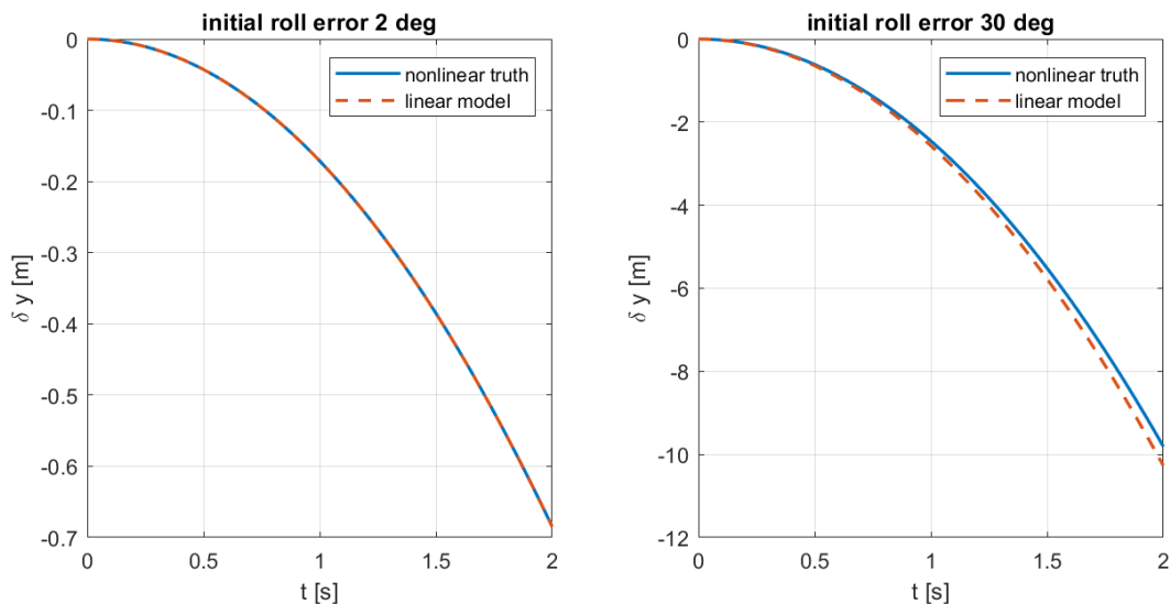
Figure 5: Sideways error \delta y after an initial roll error: nonlinear truth (solid) and linear model (dashed).
