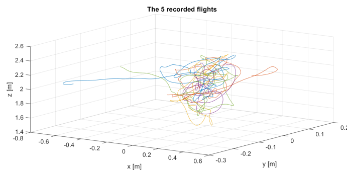
Figure 9: The five recorded flights around the hover point.
