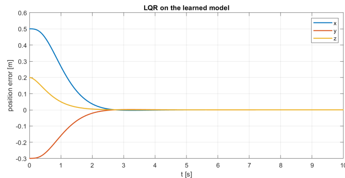
Figure 12: LQR on the learned model: the position errors die out smoothly.
