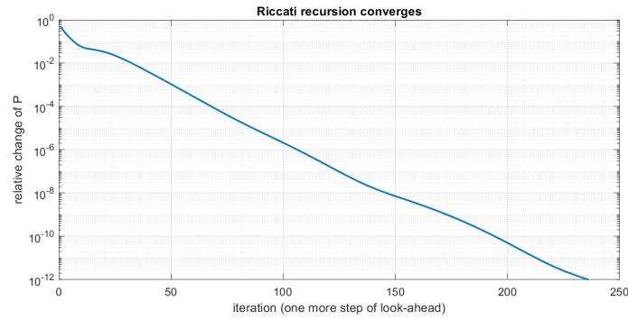
Figure 11: Riccati recursion for the drone: the change of P falls steadily until it has converged.
