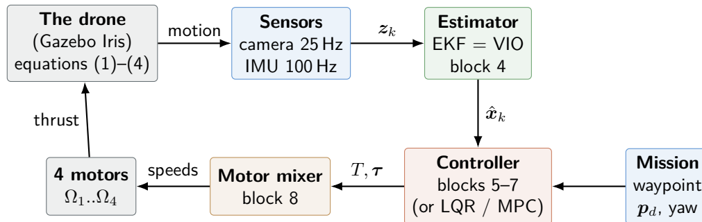
Figure 1: The closed loop. The drone moves, the sensors measure it, the estimator works out the state \hat{x} , the controller compares it with the mission and decides thrust T and torque \tau , the mixer turns that into four motor speeds, and the drone moves again. This repeats every 40 ms (25 Hz).
