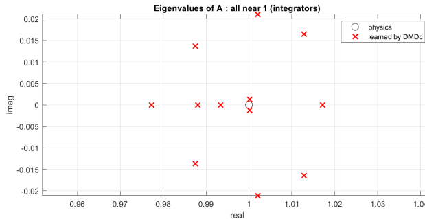
Figure 10: Eigenvalues of the learned A (crosses) and of the physics (circles). All lie at or very near 1: a chain of integrators, exactly as block 3 of Model 1 predicted.
