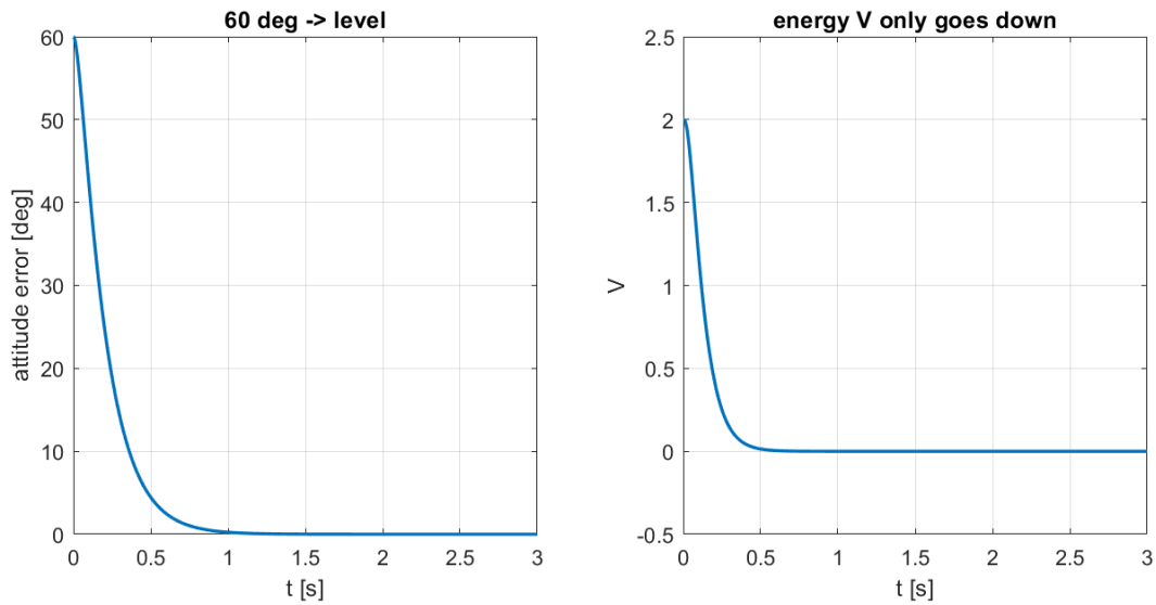
Figure 7: Block 7 alone: from 60° to level. Right: the energy V only goes down, as the proof promised.
