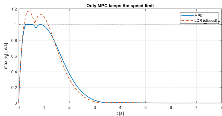
Figure 13: Largest speed component over time: only MPC respects max_velocity = 1 m/s .
