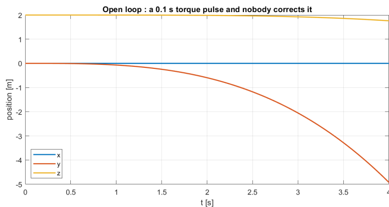
Figure 4: Open loop: a 0.1 s torque pulse and no correction. The drone slides further and further away.
