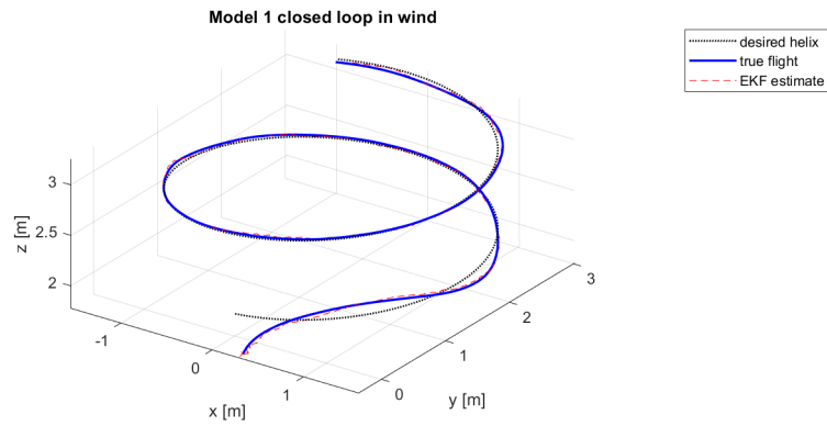
Figure 8: The complete Model 1 loop in wind: desired helix (dotted), true flight (blue), EKF estimate (red, dashed).
