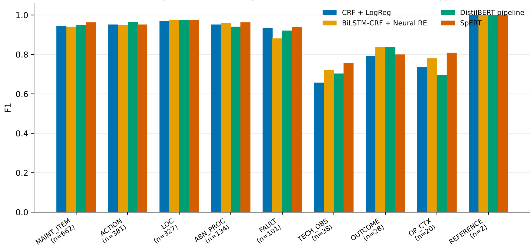
Per-class entity F1 — Full 9-entity / 11-relation schema (frozen TEST support)
