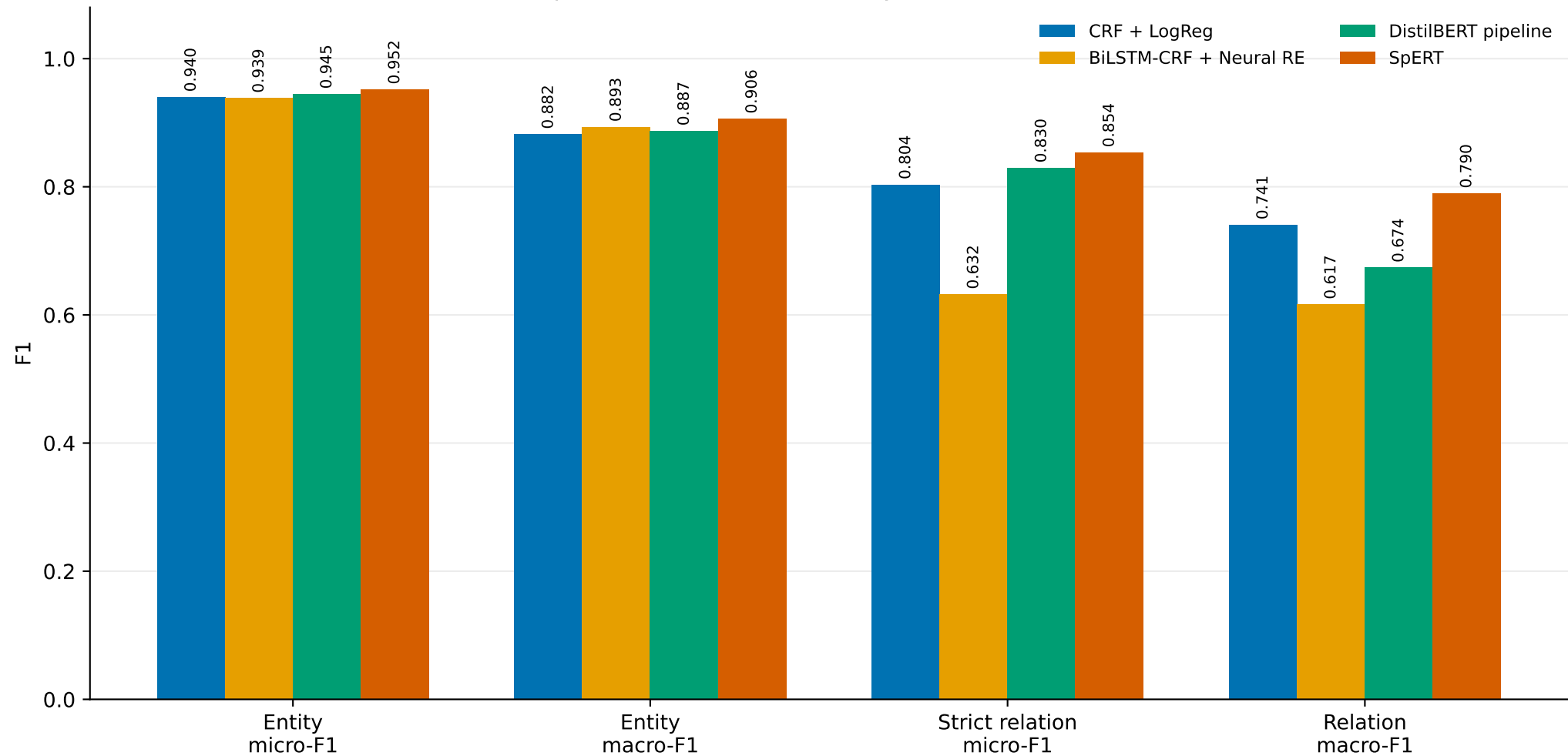
Aviation IE overall performance — Full 9-entity / 11-relation schema (frozen TEST)
