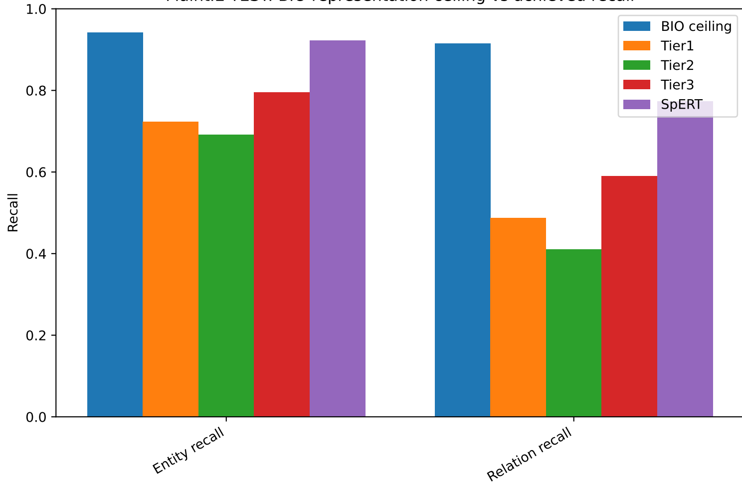
MaintIE TEST: BIO representation ceiling vs achieved recall
